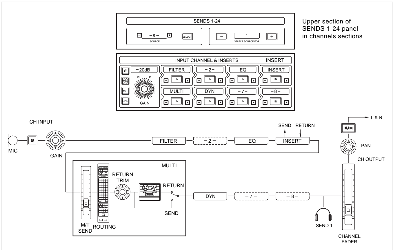
Send 1 - Pre Fader headphones feed for Foldback
