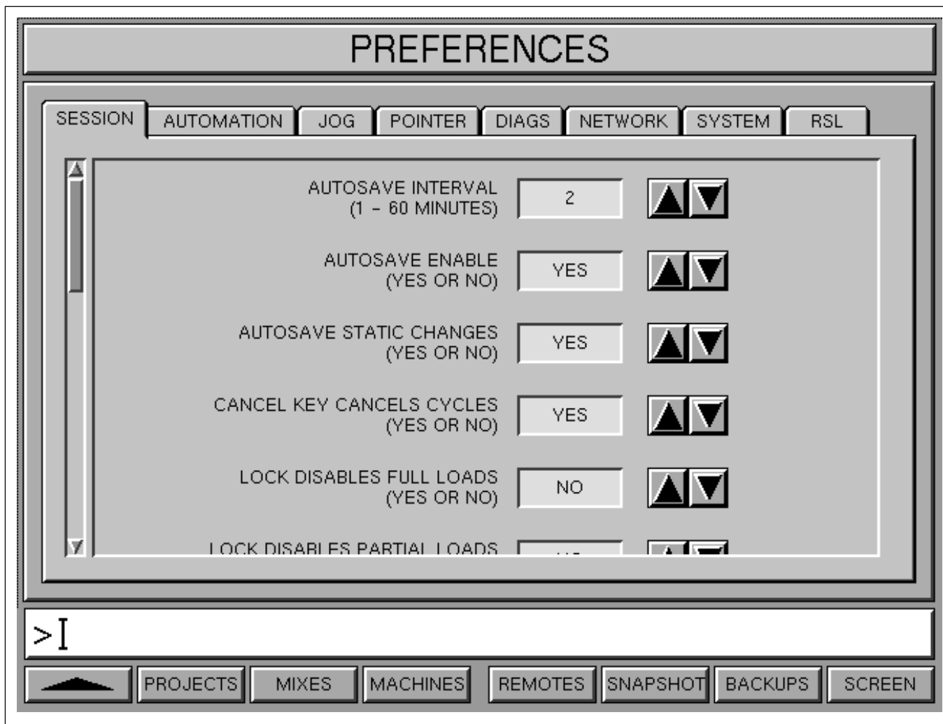
PREFERENCES screen
