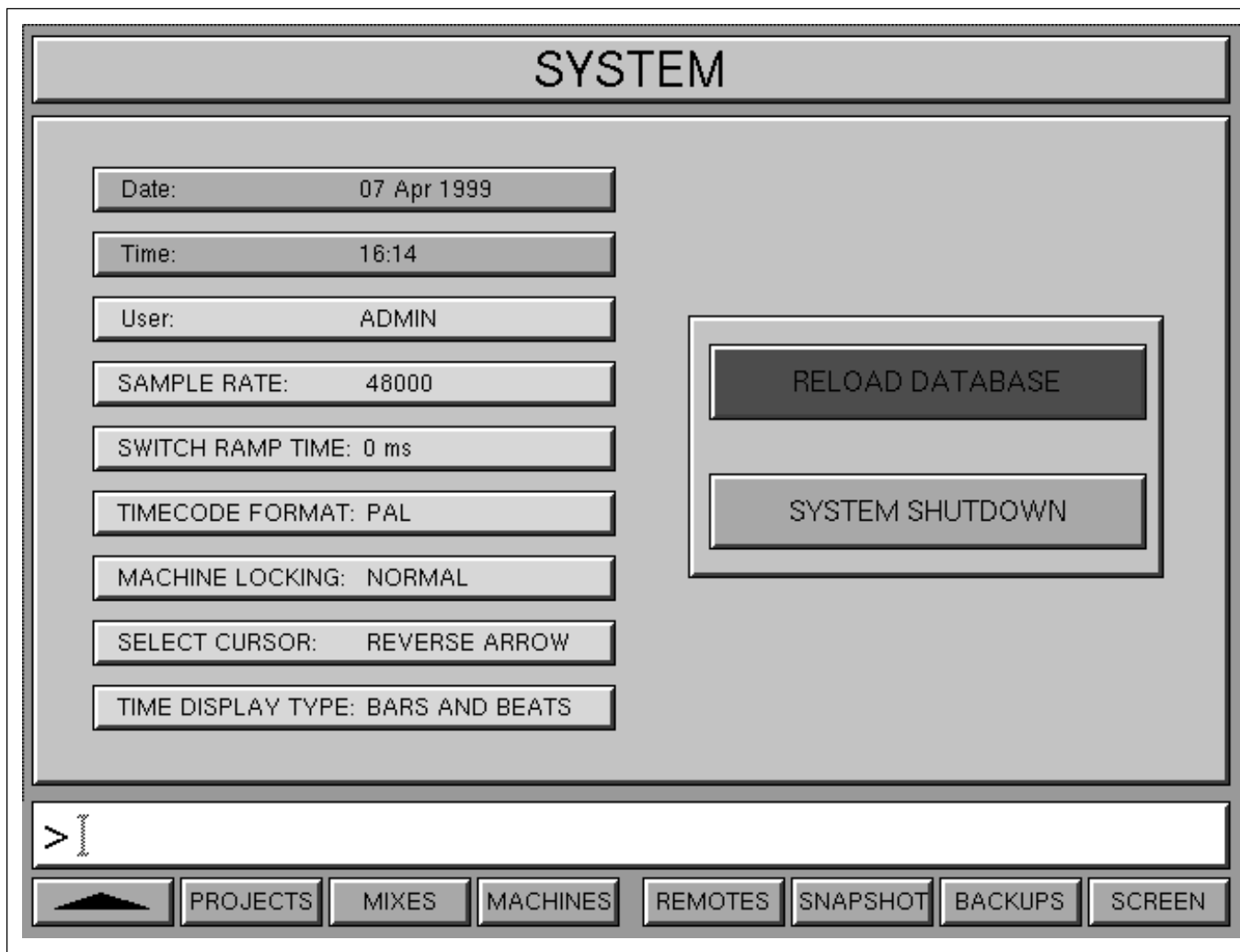
SYSTEM screen
