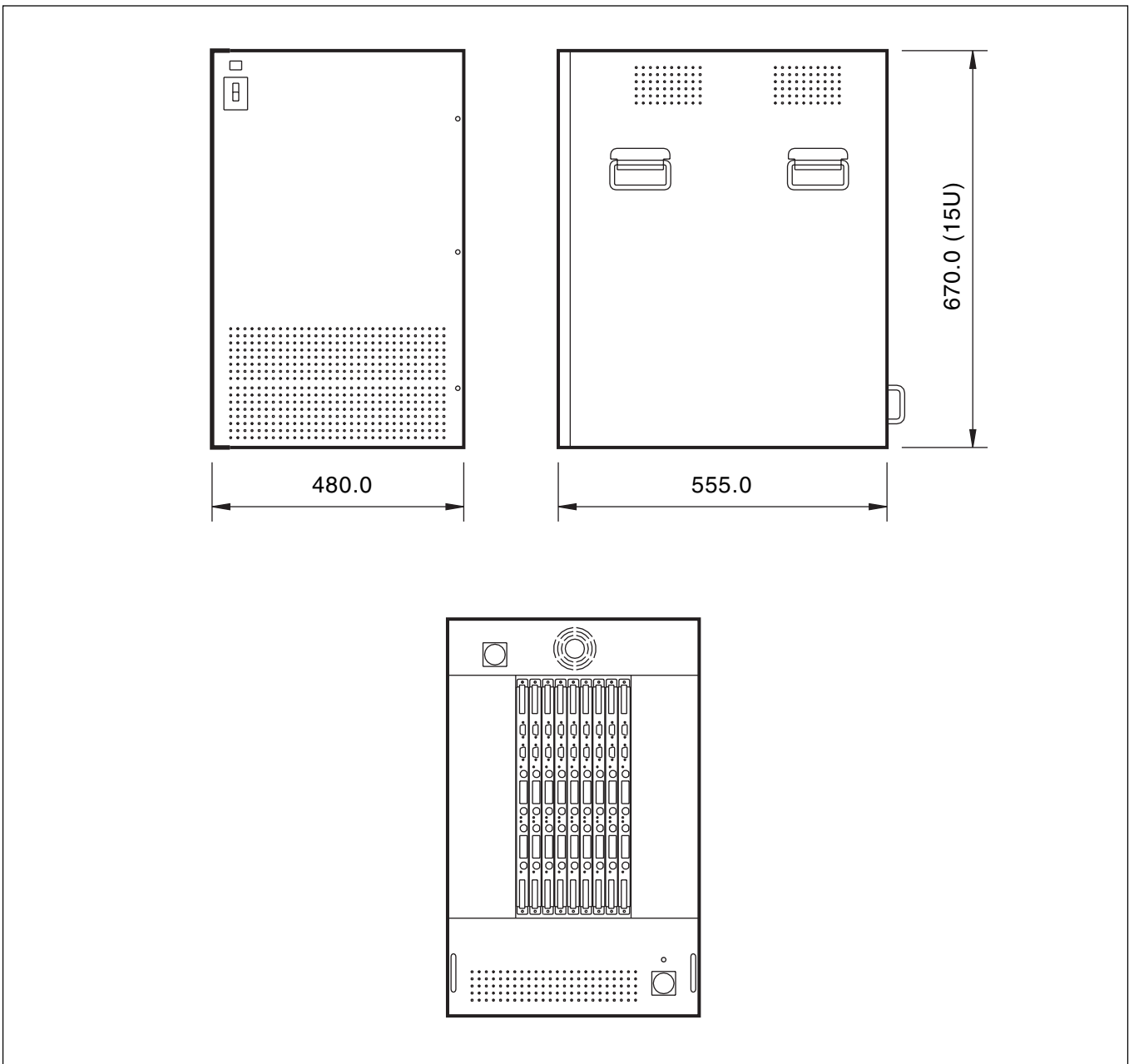
SP Rack
