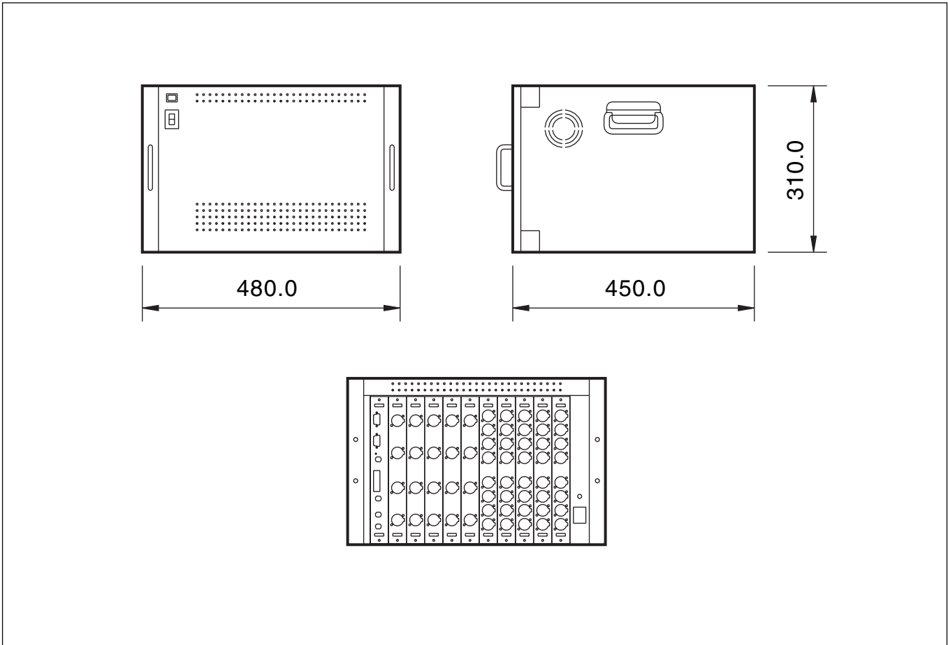
I/O Rack
