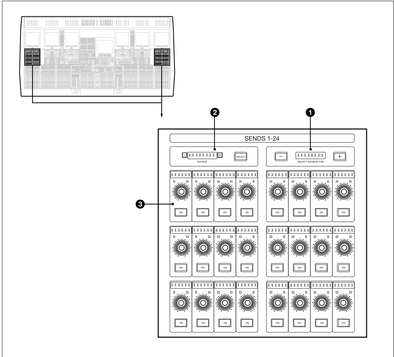
SENDS 1-24 panel
